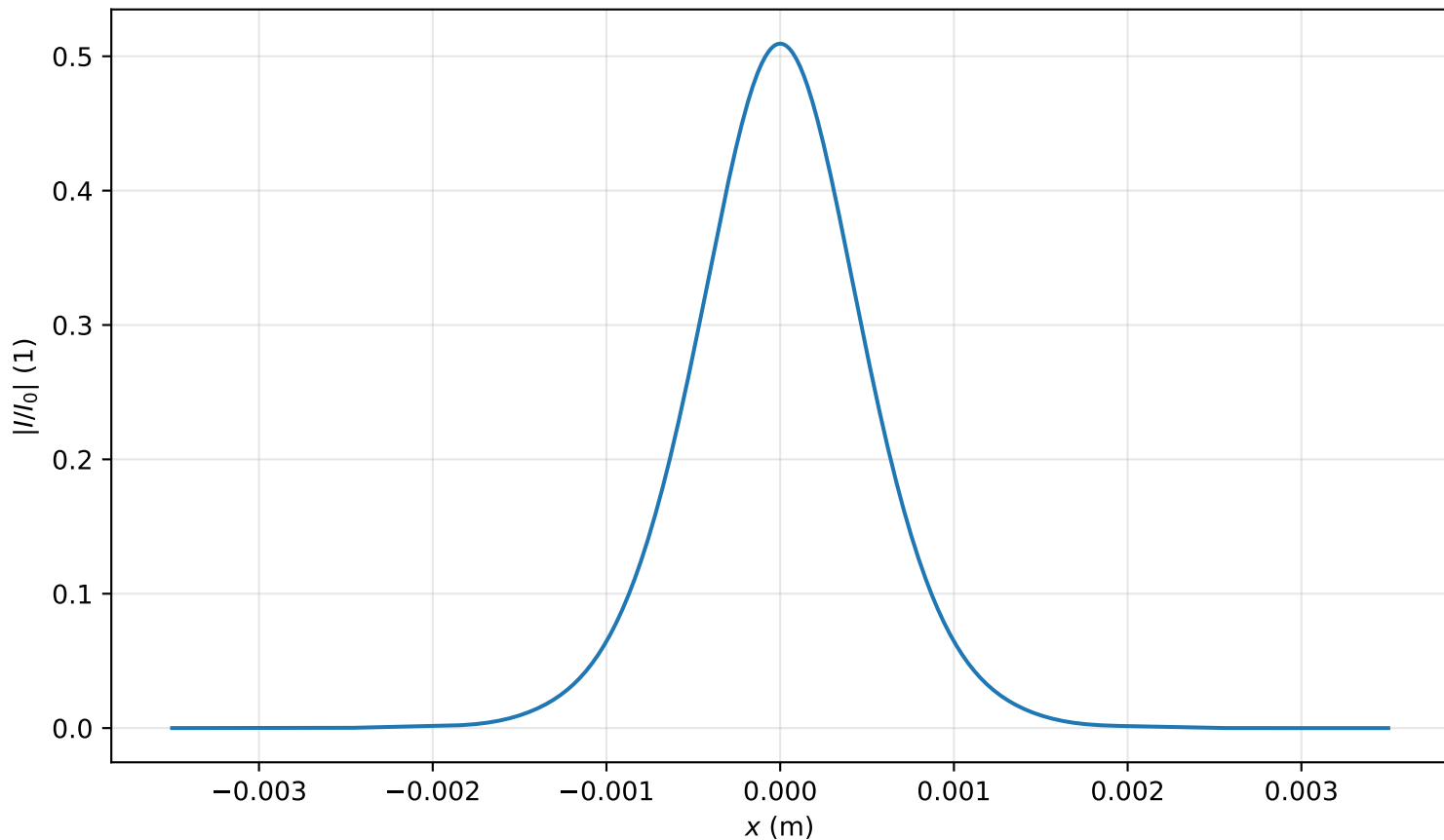
Intensity profile I(x, y = 0, z = 3.821m)/I_0 , P_{in}=0.6P_{cr} , artificial time
